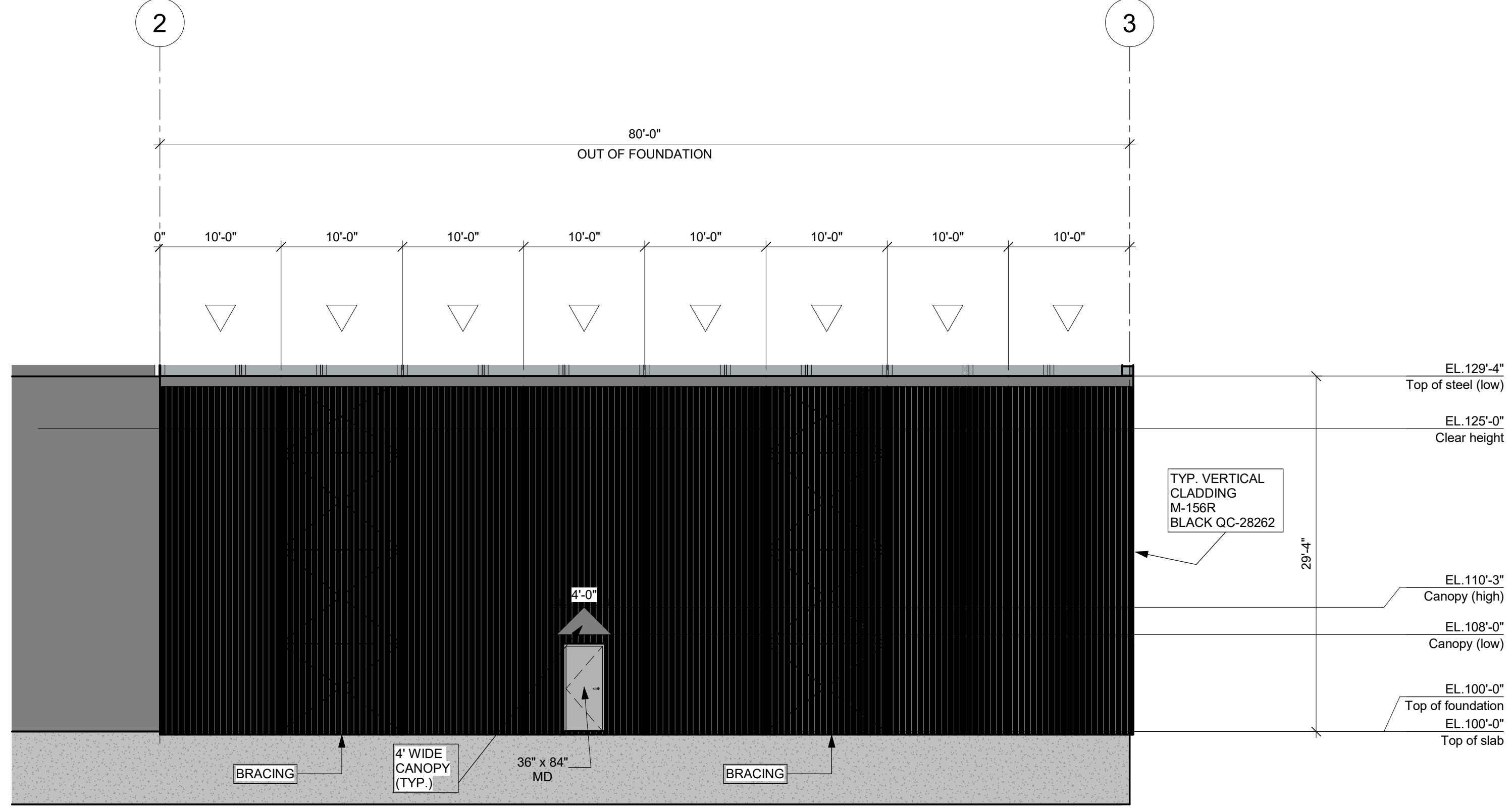
ELEVATION LINE A (NORTH) 1/8" = 1'-0"
