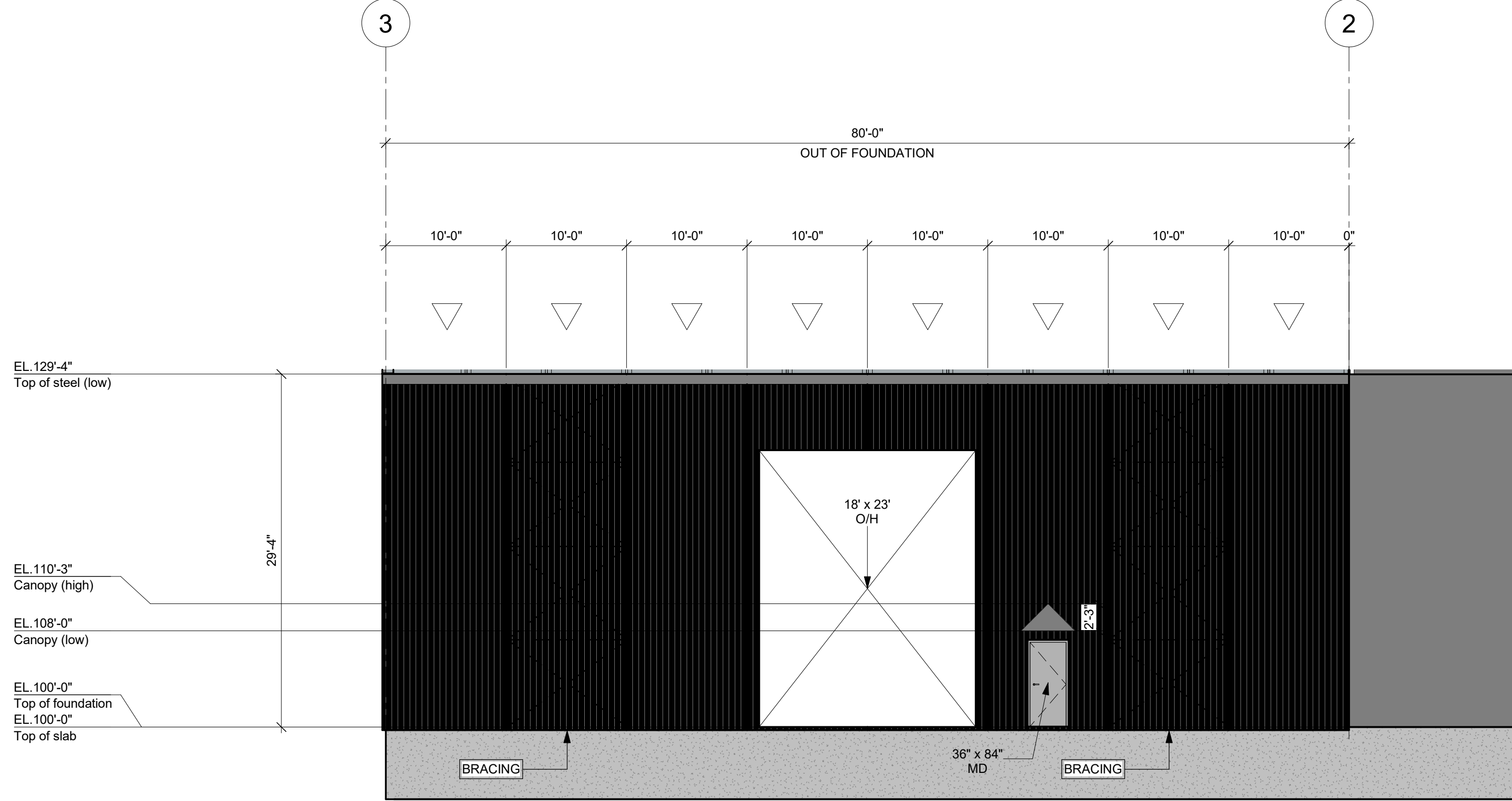
ELEVATION LINE B (SOUTH) 1/8" = 1'-0"
