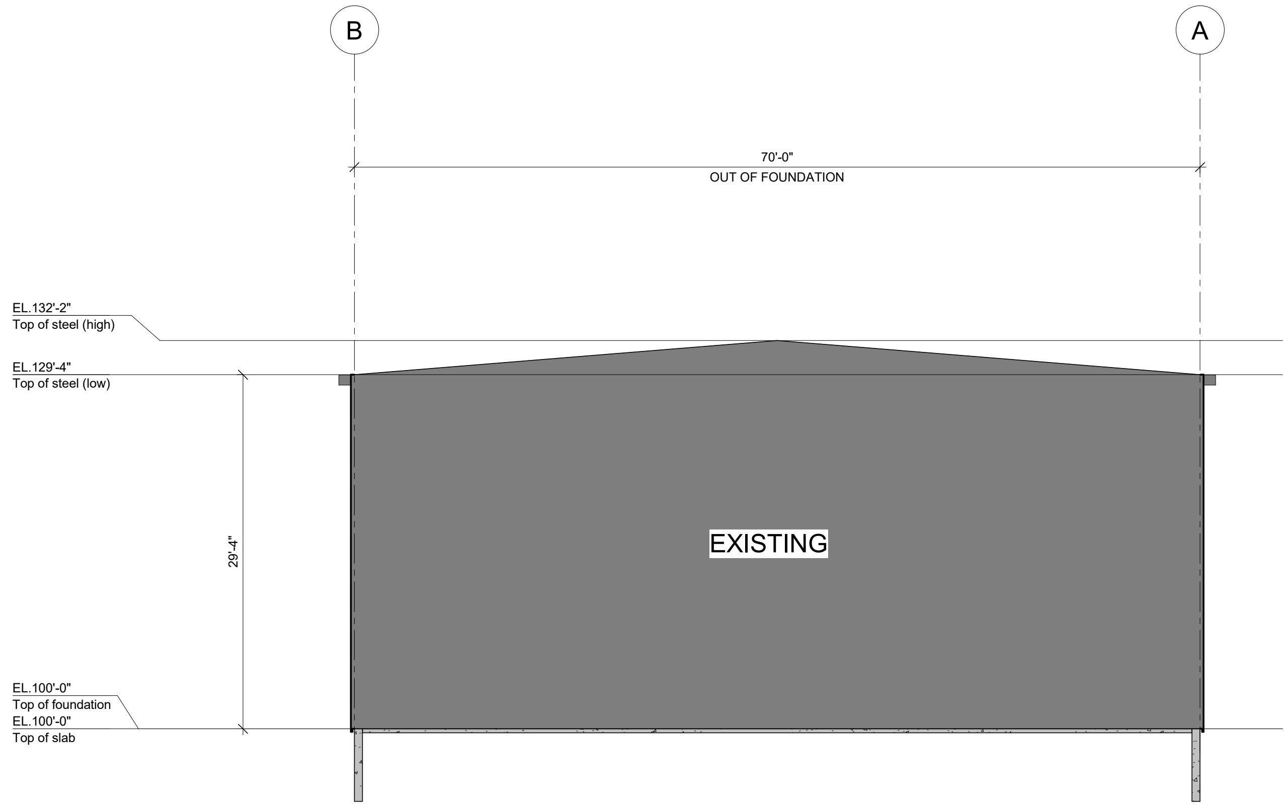
ELEVATION LINE 2 (EAST)(EXISTING) 1/8" = 1'-0"
