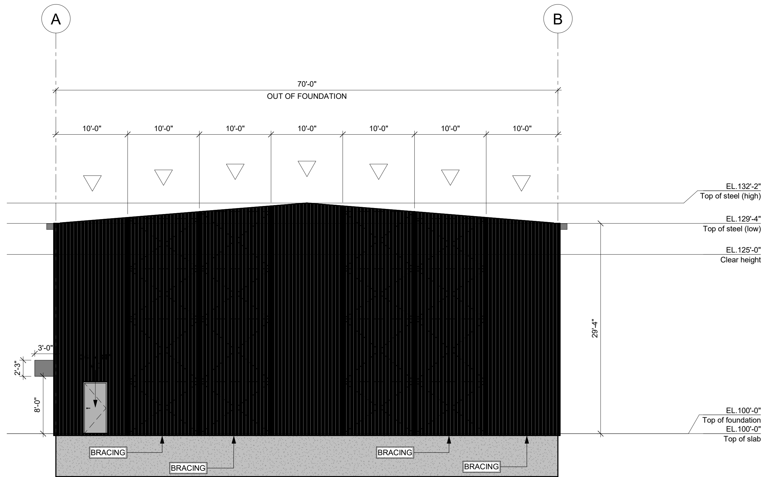
ELEVATION LINE 3 (WEST) 1/8" = 1'-0"
